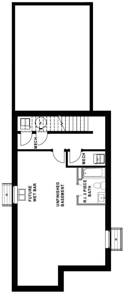
UNFINISHED BASEMENT 877 SQ.FT.
