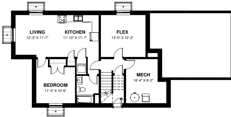
BASEMENT SUITE 580 SQ.FT. (OPTION)
