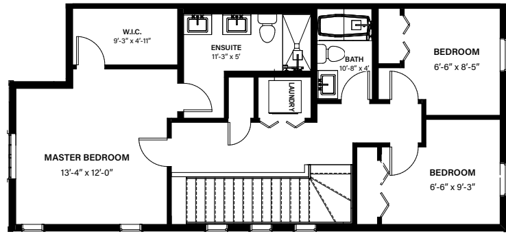
SECOND 786 SQ. FT.
