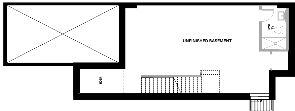
UNFINISHED BASEMENT 784 SQ. FT. Garage 307 SQ. FT.
