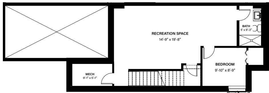
BASEMENT 784 SQ. FT.
