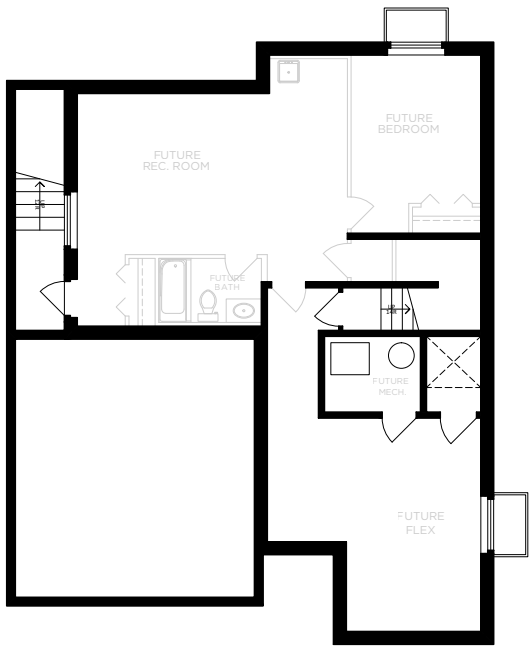
Unfinished Basement 1,126 SQ.FT.
