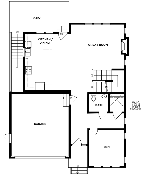
Main 1,126 SQ.FT. Garage 415 SQ. FT.
