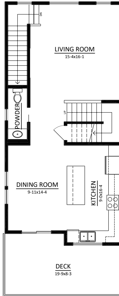
MAIN 737 SQ.FT.
