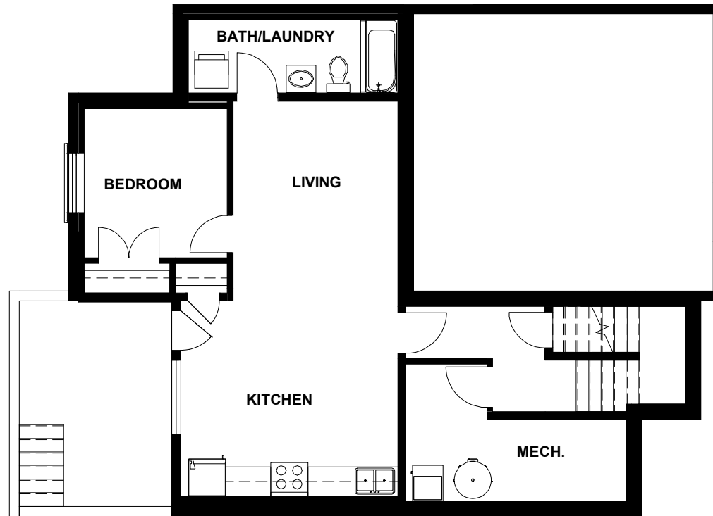
Basement Suite 648 SQ. FT. (Optional)
