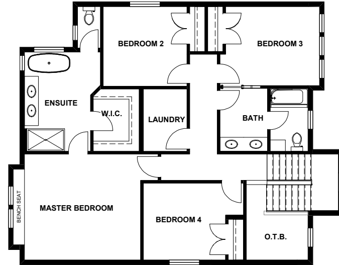
Second 1,205 SQ.FT.
