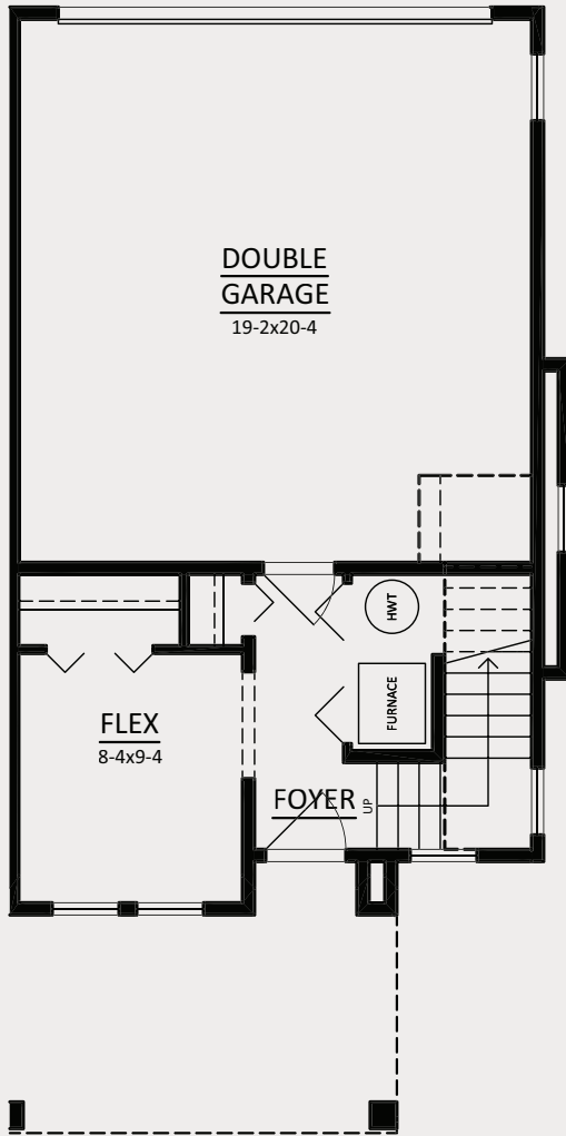
BASEMENT 232 sq. ft. GARAGE 413 sq. ft.
