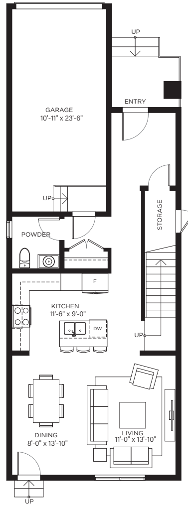
MAIN 722 SQ.FT.
