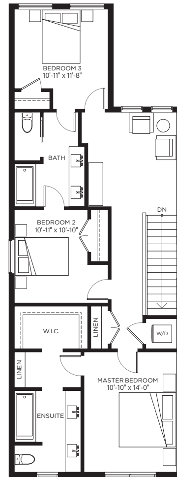
SECOND 956 SQ.FT.
