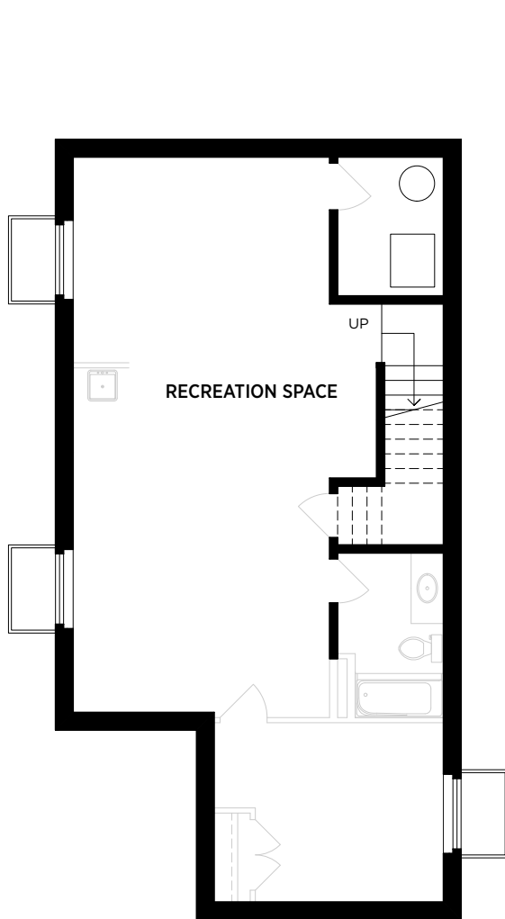
Unfinished Basement 932 SQ.FT. (Walkout, windows and doors may vary)
