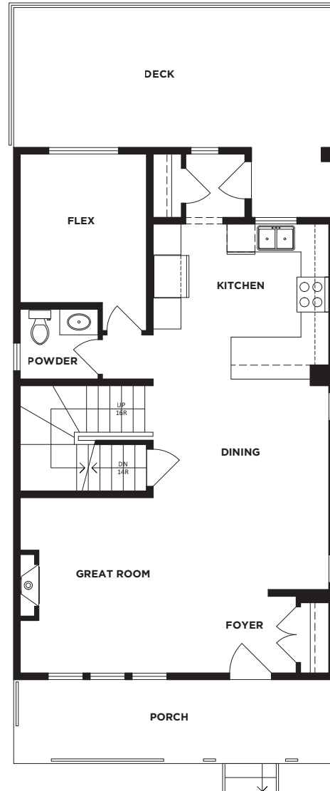
Main 844 SQ.FT.
