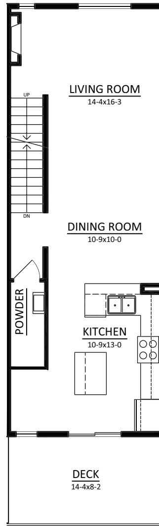
MAIN 614 SQ.FT.
