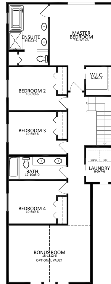
SECOND 1332 SQ.FT.
