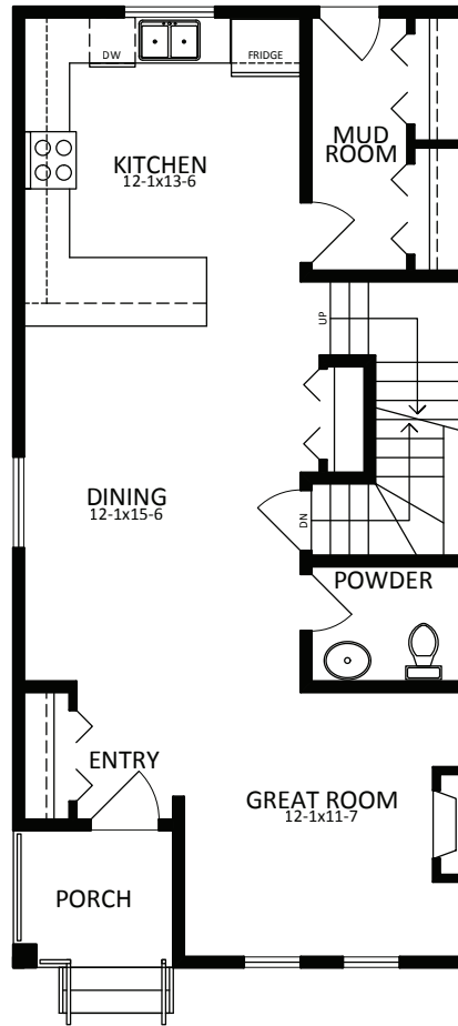
MAIN 798 SQ.FT.
