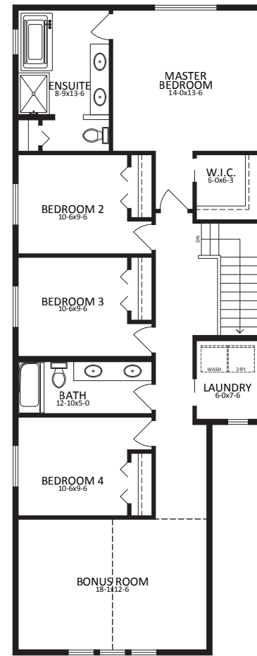
SECOND 1332 SQ.FT.
