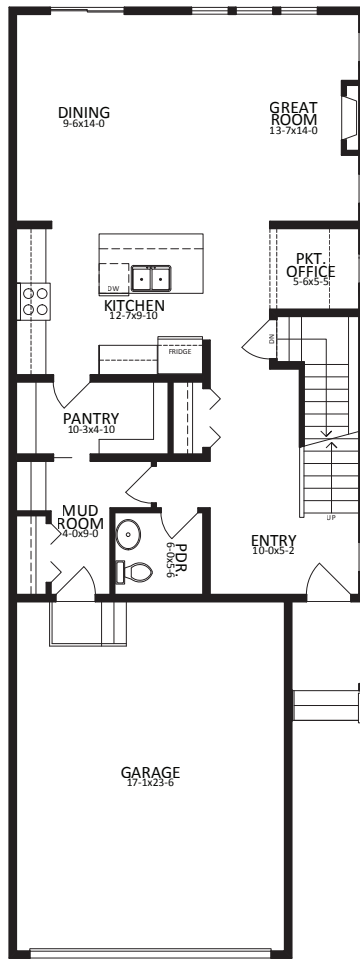
MAIN 960 SQ.FT.
